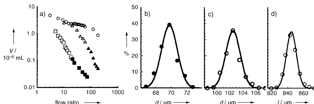
Figure 3. a) A log–log plot of the volume of the droplets versus the ratio of the rates of flow of the aqueous and monomer phases (water:monomer): dimethacrylate oxypropyldimethylsiloxane (circles); divinyl benzene (triangles); TPGDA (squares). The rate of flow of the monomer was 0.04 \text{ mL h}^{-1} . Open symbols represent disks, filled symbols correspond to spheres. b) and c) Distribution of diameters ( d ) of poly(TPGDA) spheres and disks, respectively, and d) length ( l ) of rods. The experimental points were fitted with a Gaussian distribution. The resulting polydispersities are 1.5% for spheres, 1.1% for disks, and 1% for rods.
